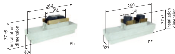
Wear height of the carbon brushes 20 mm
