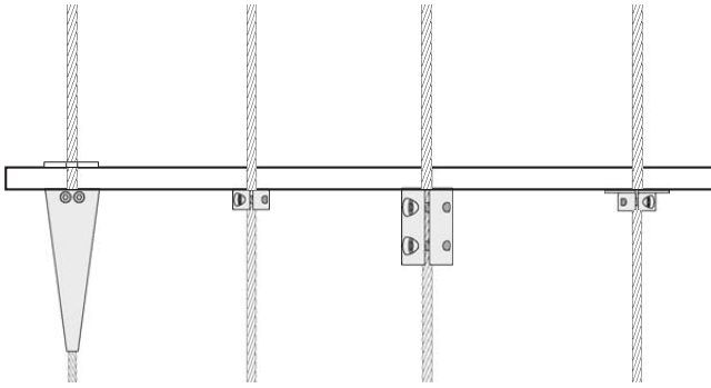
Cable cone clamp with cover disc, light clamp ring, clamp ring, light clamp ring with support for horizontal hanging of shelves and tablets.
