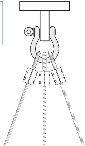
Loop clamps attached to bow shackle.
