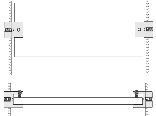
Double cable junction with clamping holder for horizontal and vertical hanging of displays and shelves.
