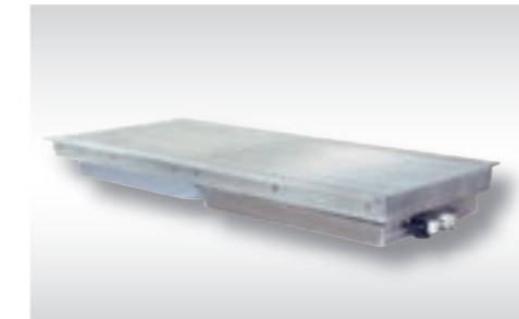
- Pick-up system with integrated power electronics - Additional 24 VDC output as auxiliary voltage - Parallel connection of several pick-up systems possible
