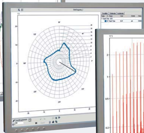
Orbit-diagram
