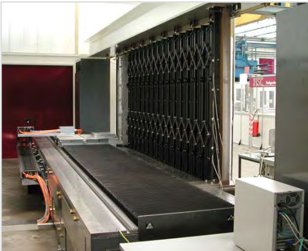
Traverse test on a slat cover with shearing system at the PTW: force sensors measure the vibrations during traverses to block size.
