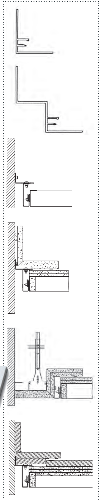
Randabschlüsse F0, F30, F90
