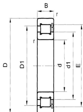
NCF V
