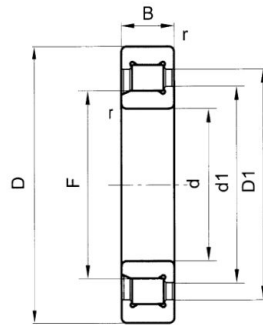
NJ V
