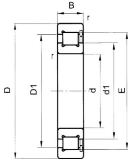
NCF V
