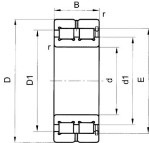
NNCF V
