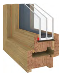
Overlap Bonding Ködiglaze ADG / SDG Wooden Window
