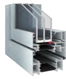
Glass Edge Bonding Ködiglaze SDG Aluminium Window
