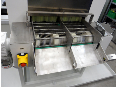
Two-lane tape guide
