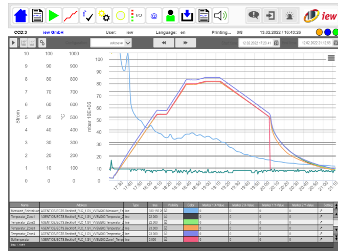
Temperature profile
