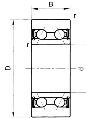
LR52-2RS LR53-2RS
