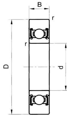
LR1-2RS LR2-2RS
