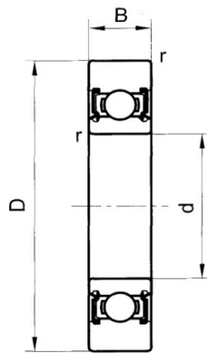
LR1-2RS LR2-2RS
