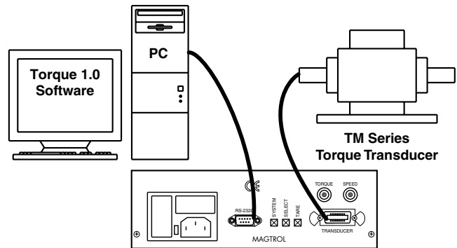
Model 3410 Torque Display PC-Based System Configuration Torque Transducer with Model 3410 Display and Torque 1.0 Software
